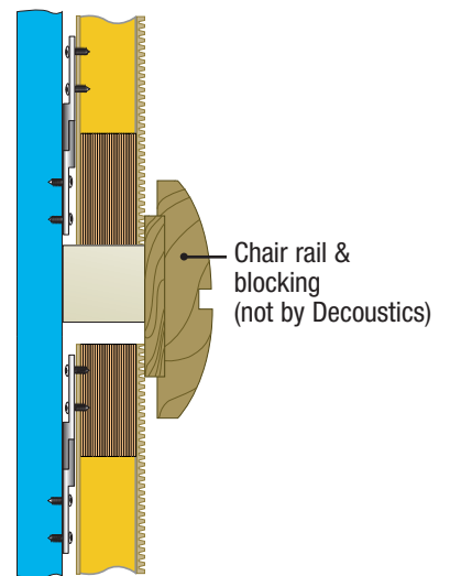
Quadrillo Wall Section Typical
