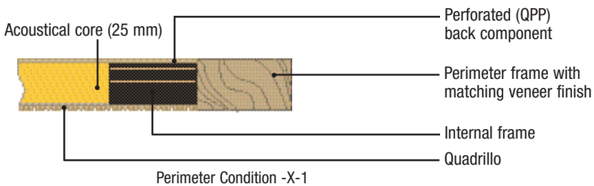
Quadrillo Details Typical
