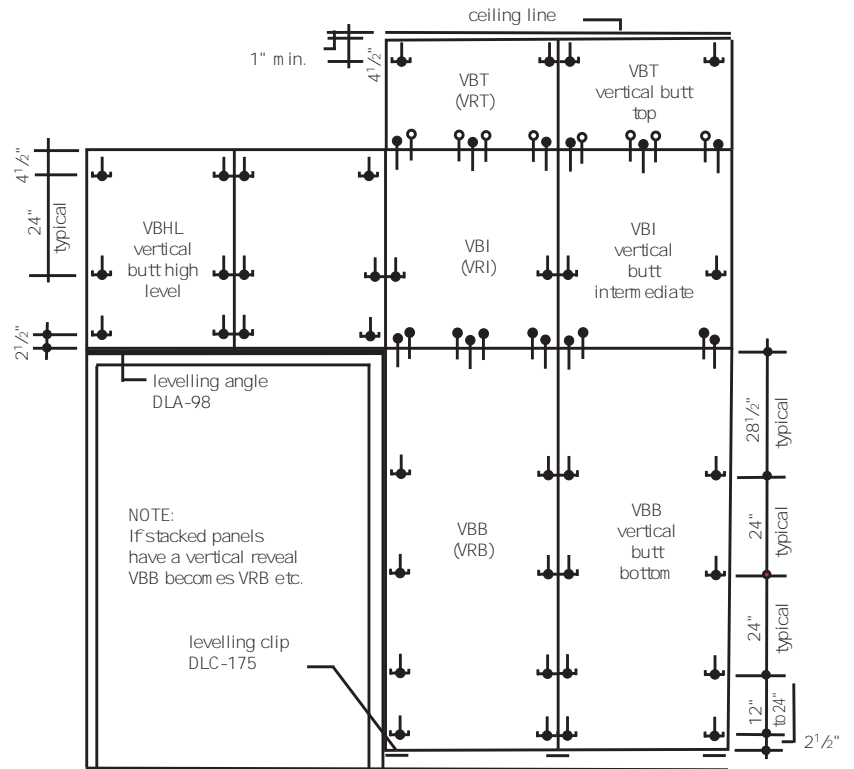
VERTICAL STACK ARRANGEMENT
