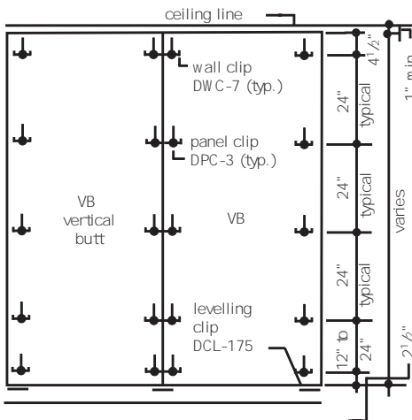
BUTT ARRANGEMENT
