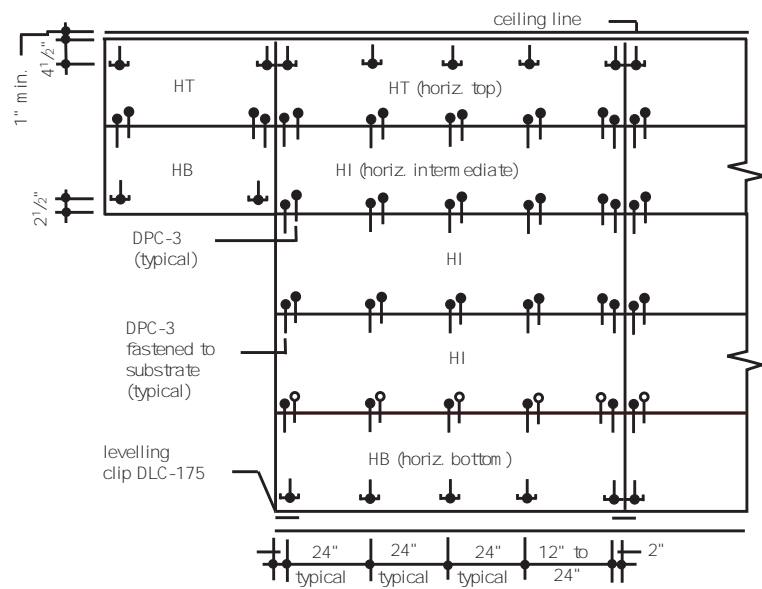
HORIZONTAL STACK ARRANGEMENT
