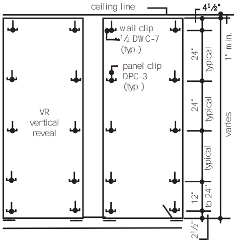
REVEAL ARRANGEMENT
